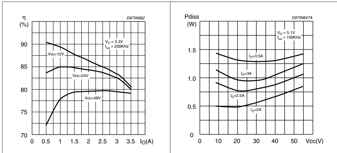
Figure 33. Power dissipation vs. output voltage (device only)
