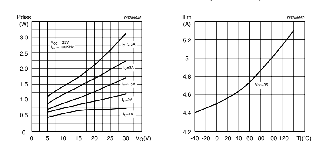
Figure 34. Pulse by pulse limiting current vs. junction temperature
